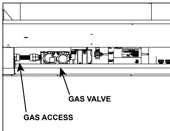
Figure 9.5. Gas Fitting Access with Vanity Panel Removed
