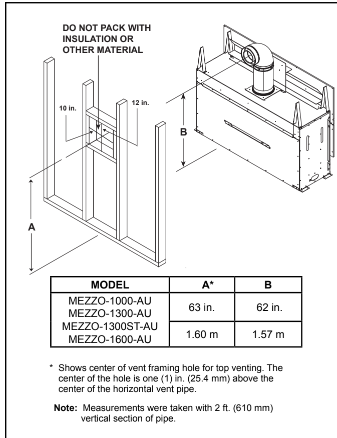
→ Figure 5.2 Wall Penetration
