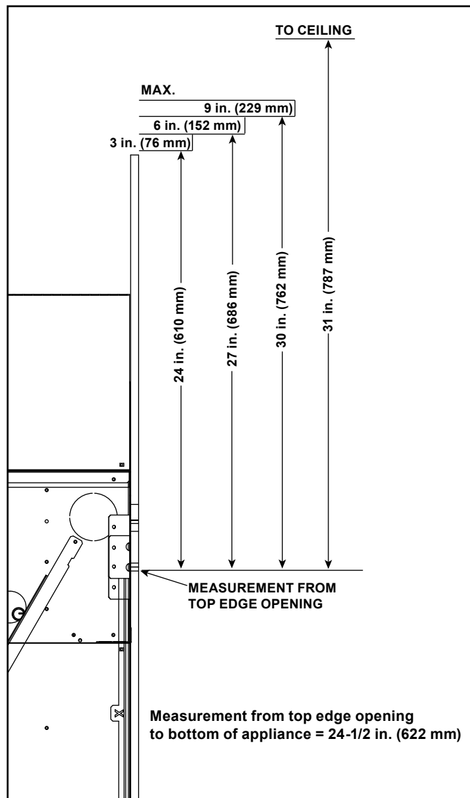
Figure 10.8 Minimum Vertical and Maximum Horizontal Dimensions of Combustibles - MEZZO-1600-AU
