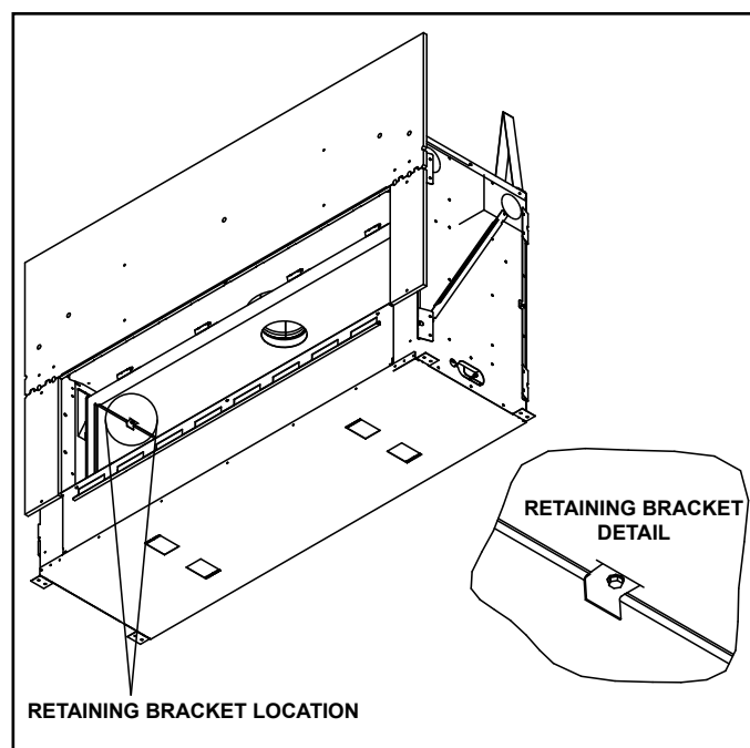
Figure 11.6 Retaining Bracket Installation - Single-sided Models
