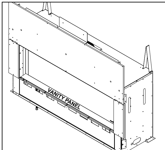
Figure 11.2 Vanity Panel Location
