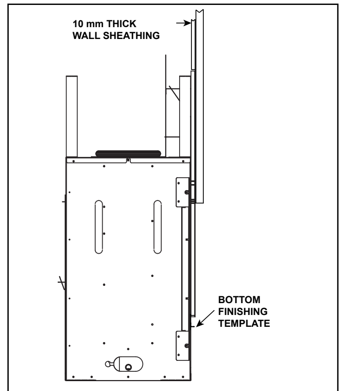
Figure 10.2 Finishing and Facing Materials - Single-sided Models
